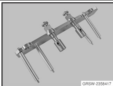
Injector Removal Tool Order P/N 83 30 2 358 417 Price - $437.58
