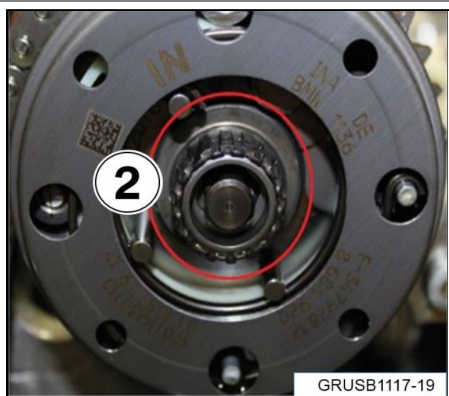
VANOS Central Valve (2) produced after 8/2017 with splined head requiring special tool P/N 83 30 2 450 487.
